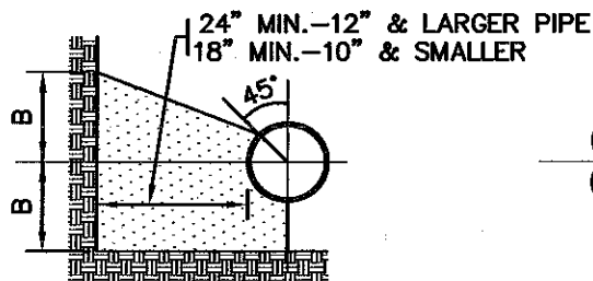
SECTION X-X BENDS & TEES
