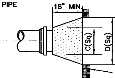
PLAN & ELEVATION PLUGS
